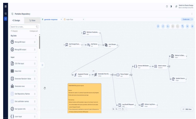
Figure 1: Drag-and-Drop Data Transformation in Pentaho Data Integration
